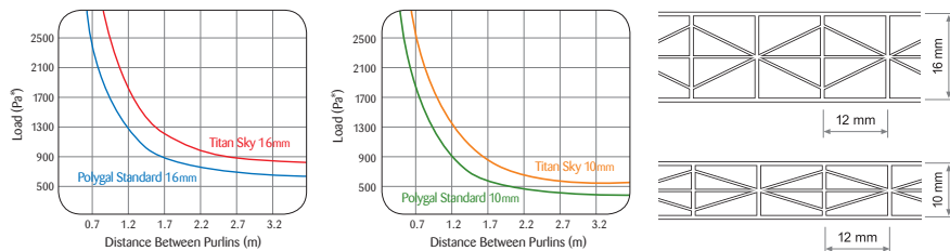
Load vs. Distance Between Purlins at an Absolute Deflection of 50 mm and Rafter Distance of 1.05m
